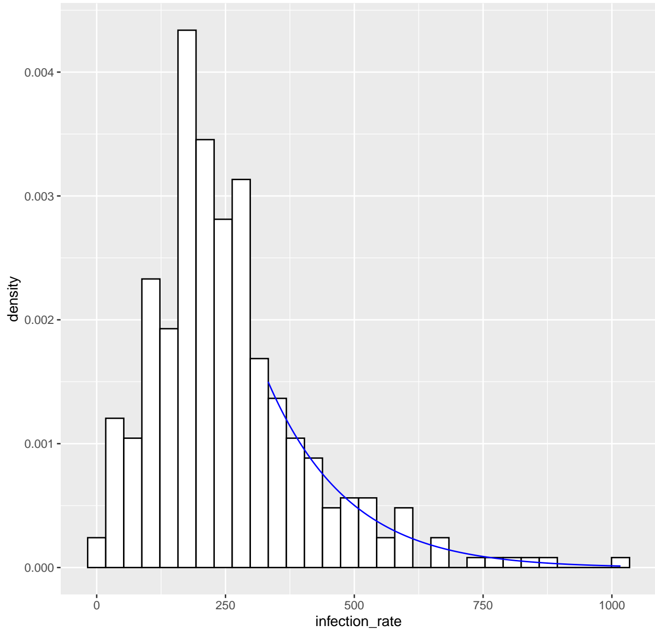
Fitted tail density GPD( 332.7 , 150.21 , -0.04 ), k= 80 -- 14-05-2020
