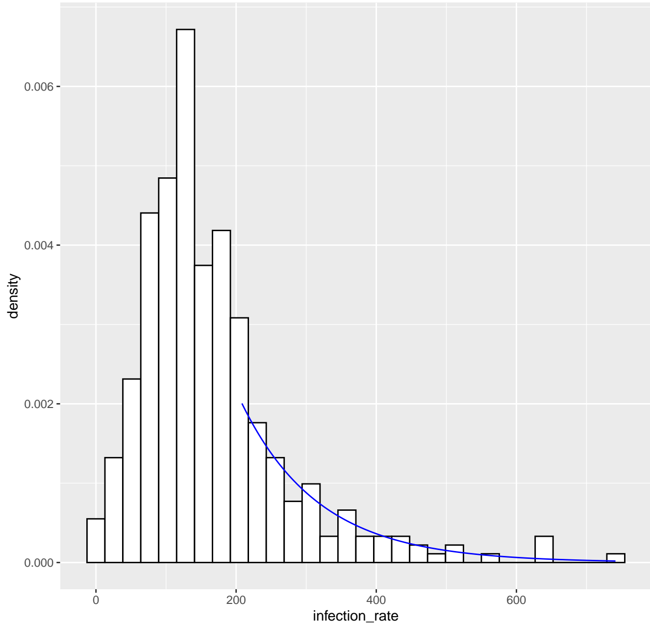
Fitted tail density GPD( 208.3 , 112.41 , 0.01 ), k= 80 -- 14-04-2020
