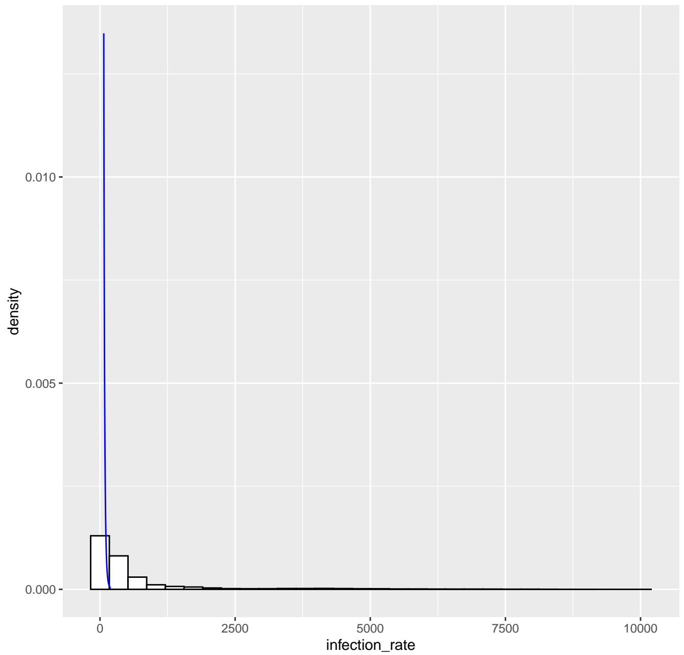
Fitted tail density GPD( 69.7 , 16.71 , 0.12 ), k= 80 -- 13-12-2022
