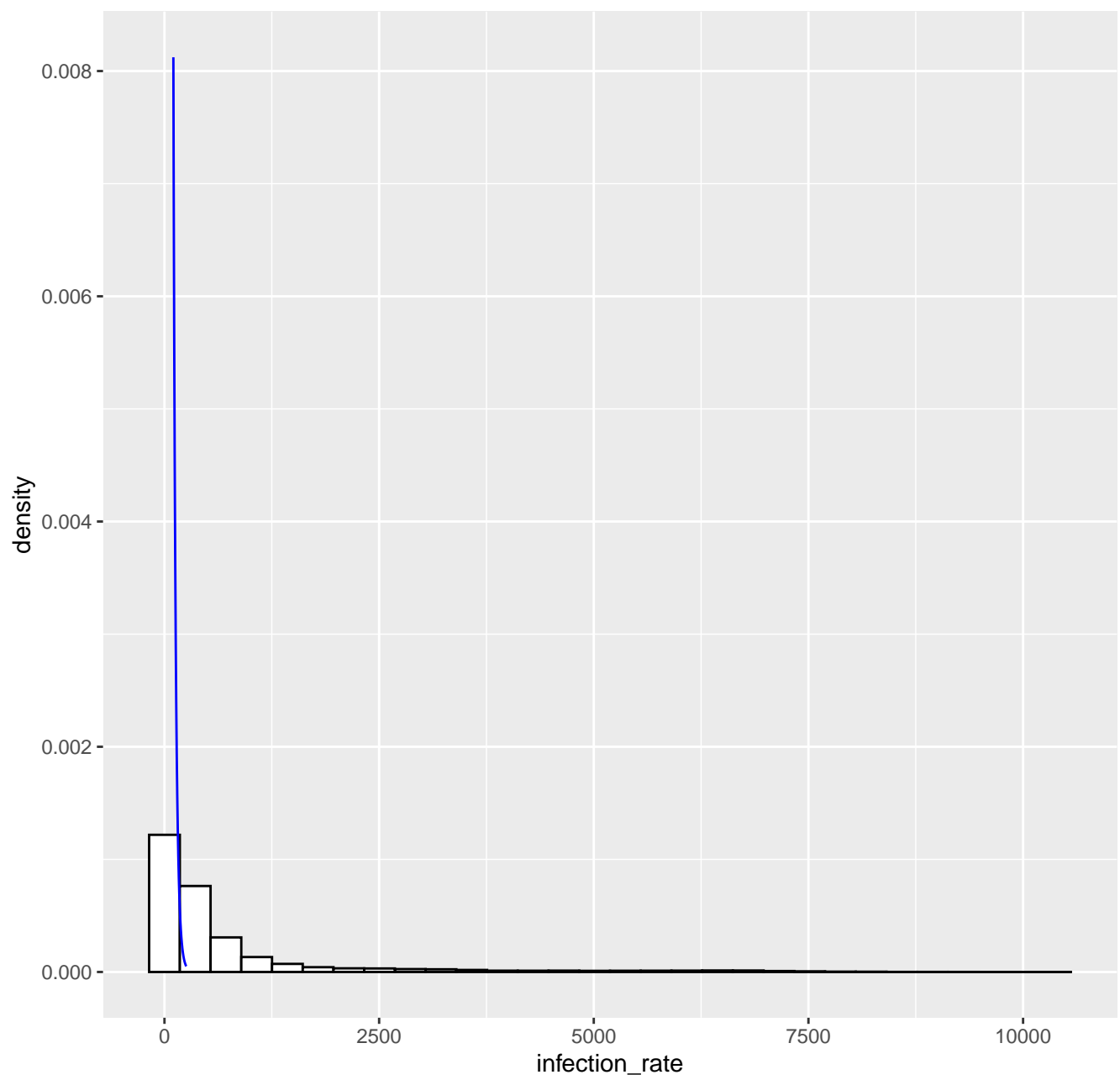
Fitted tail density GPD( 103.5 , 27.75 , 0.04 ), k= 80 -- 13-09-2022
