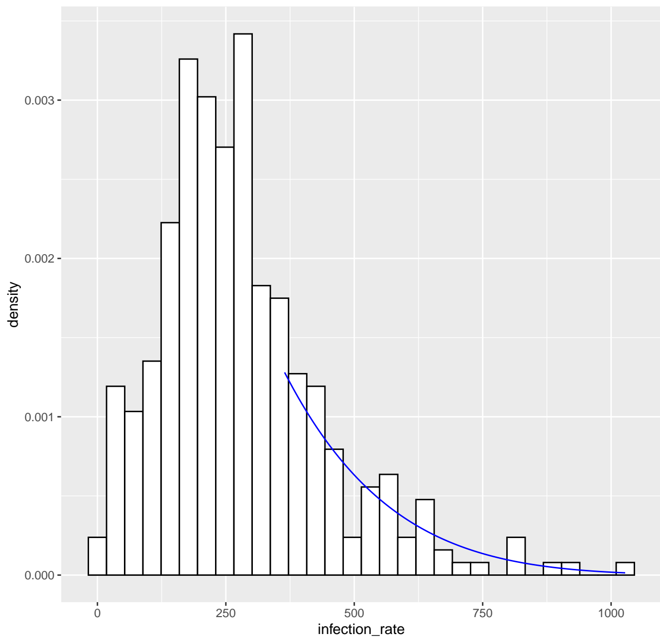
Fitted tail density GPD( 364.4 , 176.02 , -0.13 ), k= 80 -- 13-06-2020
