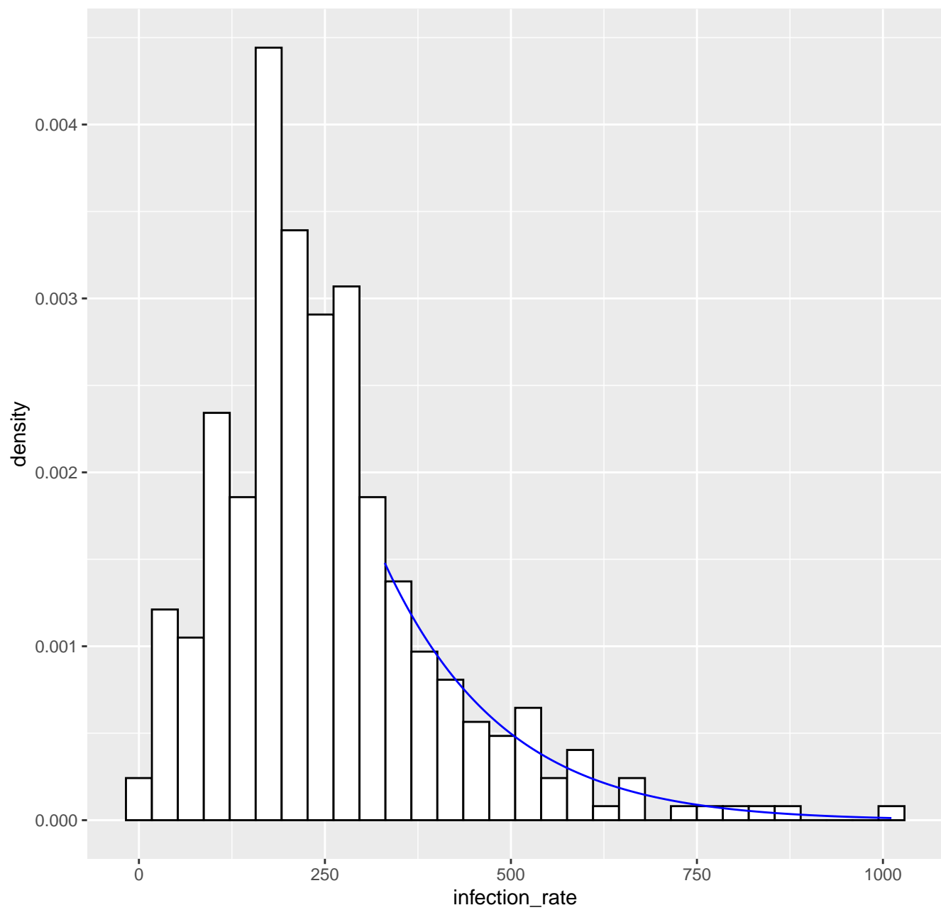
Fitted tail density GPD( 330.4 , 152.33 , -0.05 ), k= 80 -- 13-05-2020
