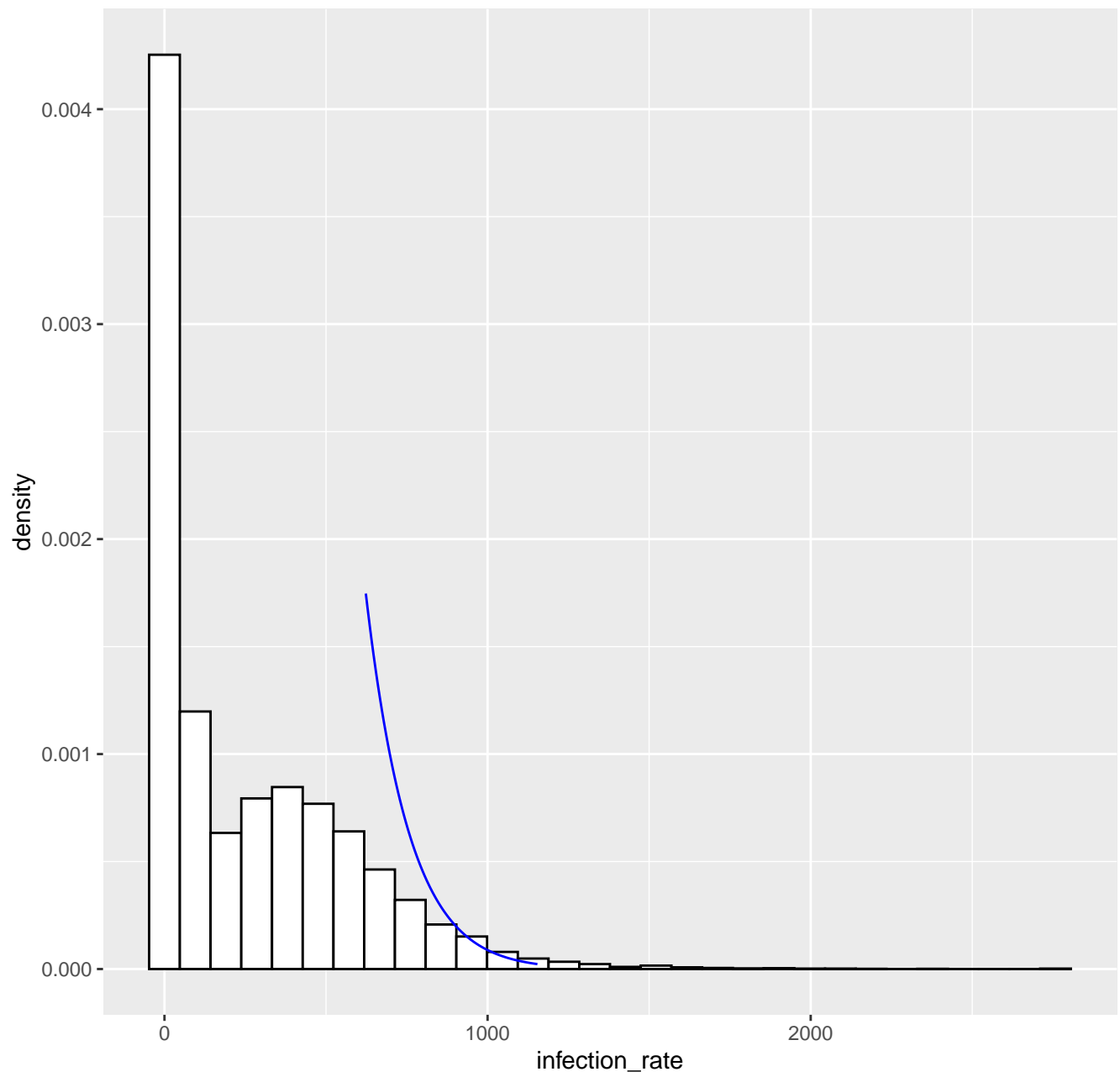
Fitted tail density GPD( 623.2 , 129.01 , -0.04 ), k= 80 -- 13-04-2021
