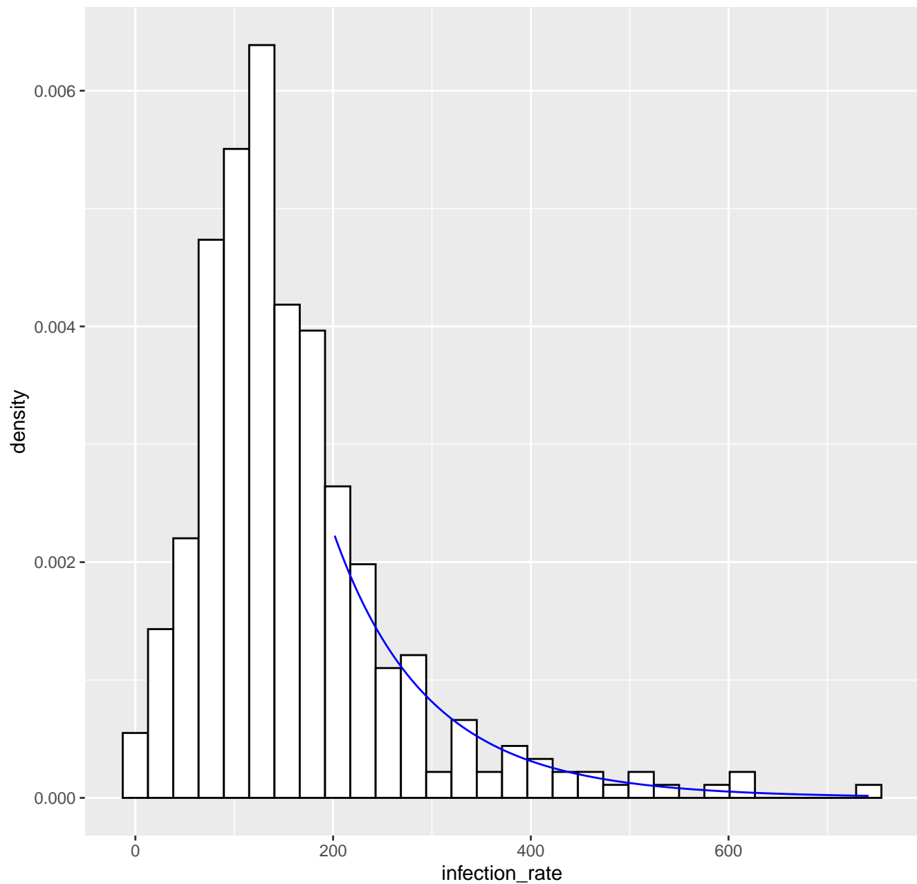
Fitted tail density GPD( 201.6 , 101.3 , 0.07 ), k= 80 -- 13-04-2020
