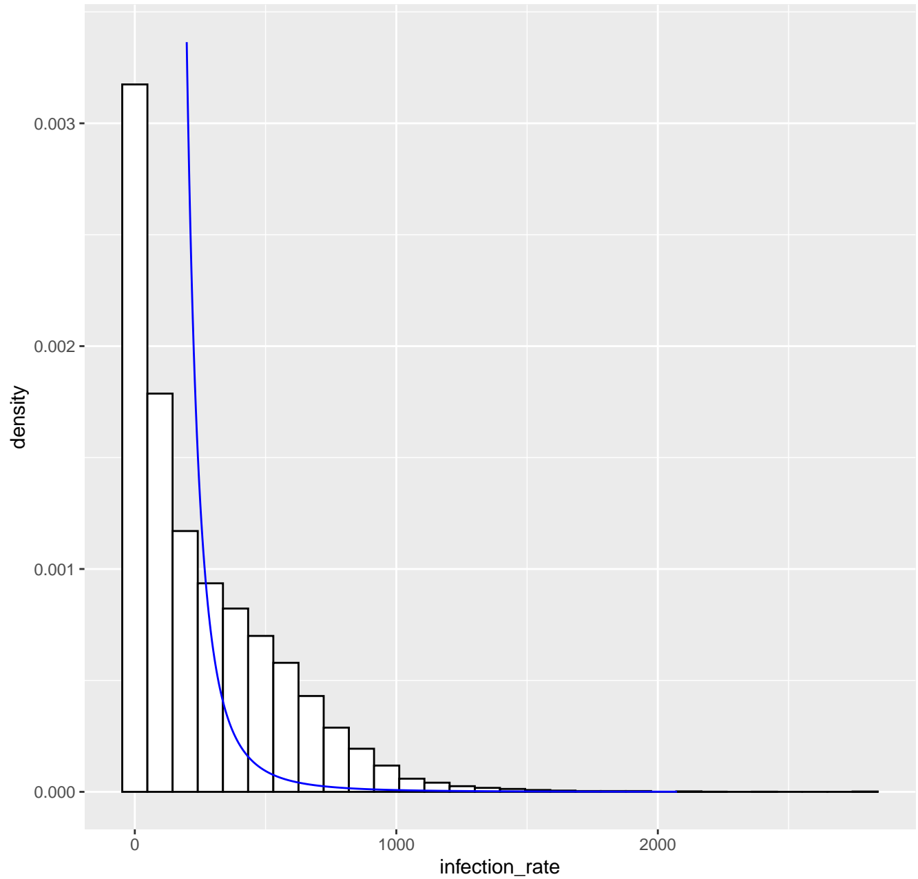
Fitted tail density GPD( 198.5 , 66.98 , 0.43 ), k= 80 -- 12-10-2021
