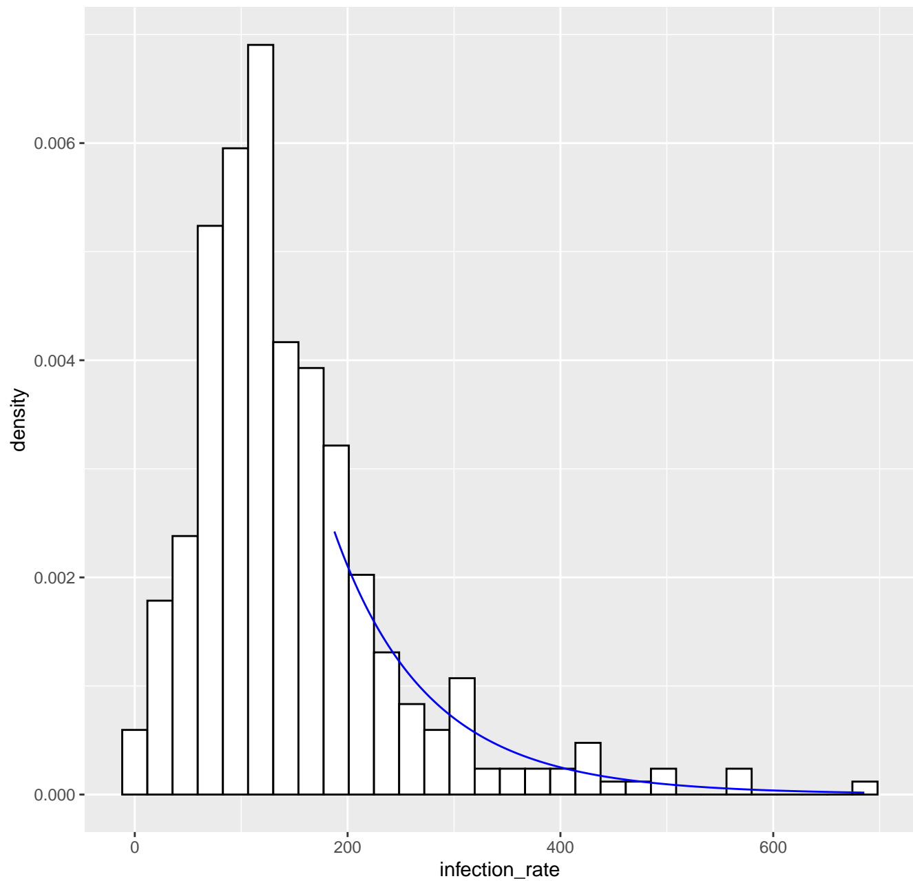
Fitted tail density GPD( 187.6 , 93.01 , 0.06 ), k= 80 -- 12-04-2020
