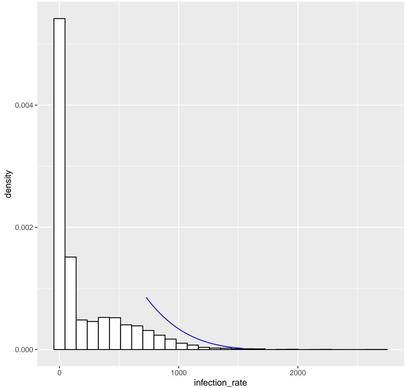
Fitted tail density GPD( 726.9 , 263.61 , -0.2 ), k= 80 -- 12-01-2021
