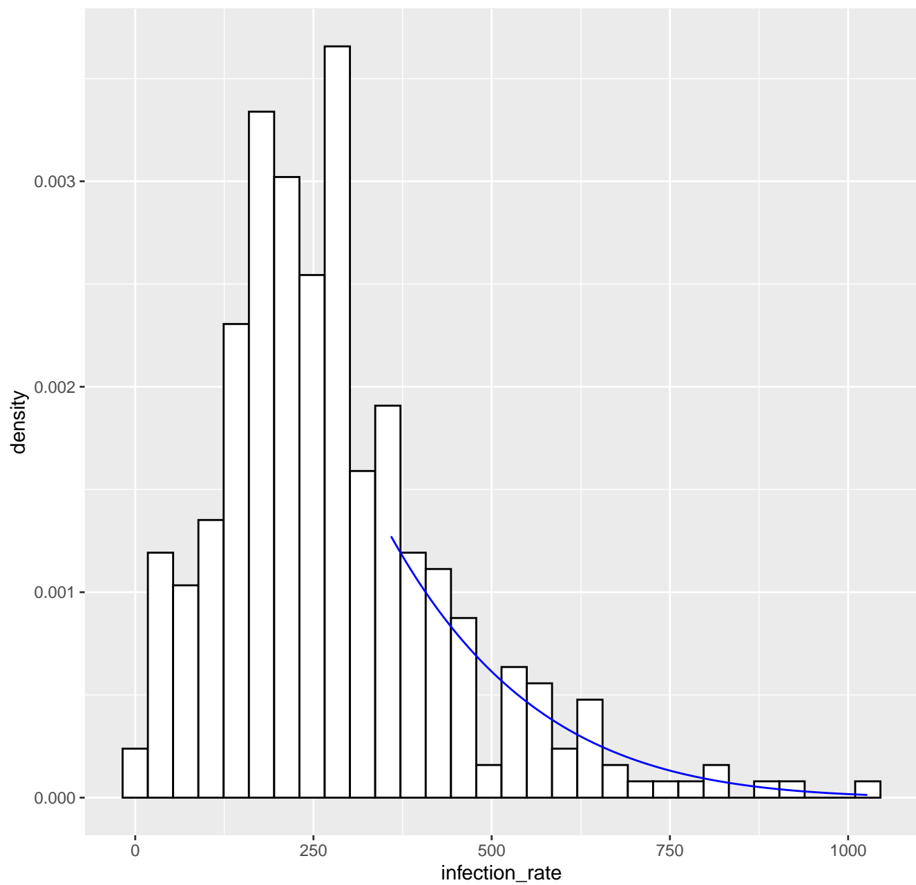
Fitted tail density GPD( 358.9 , 177.15 , -0.13 ), k= 80 -- 11-06-2020
