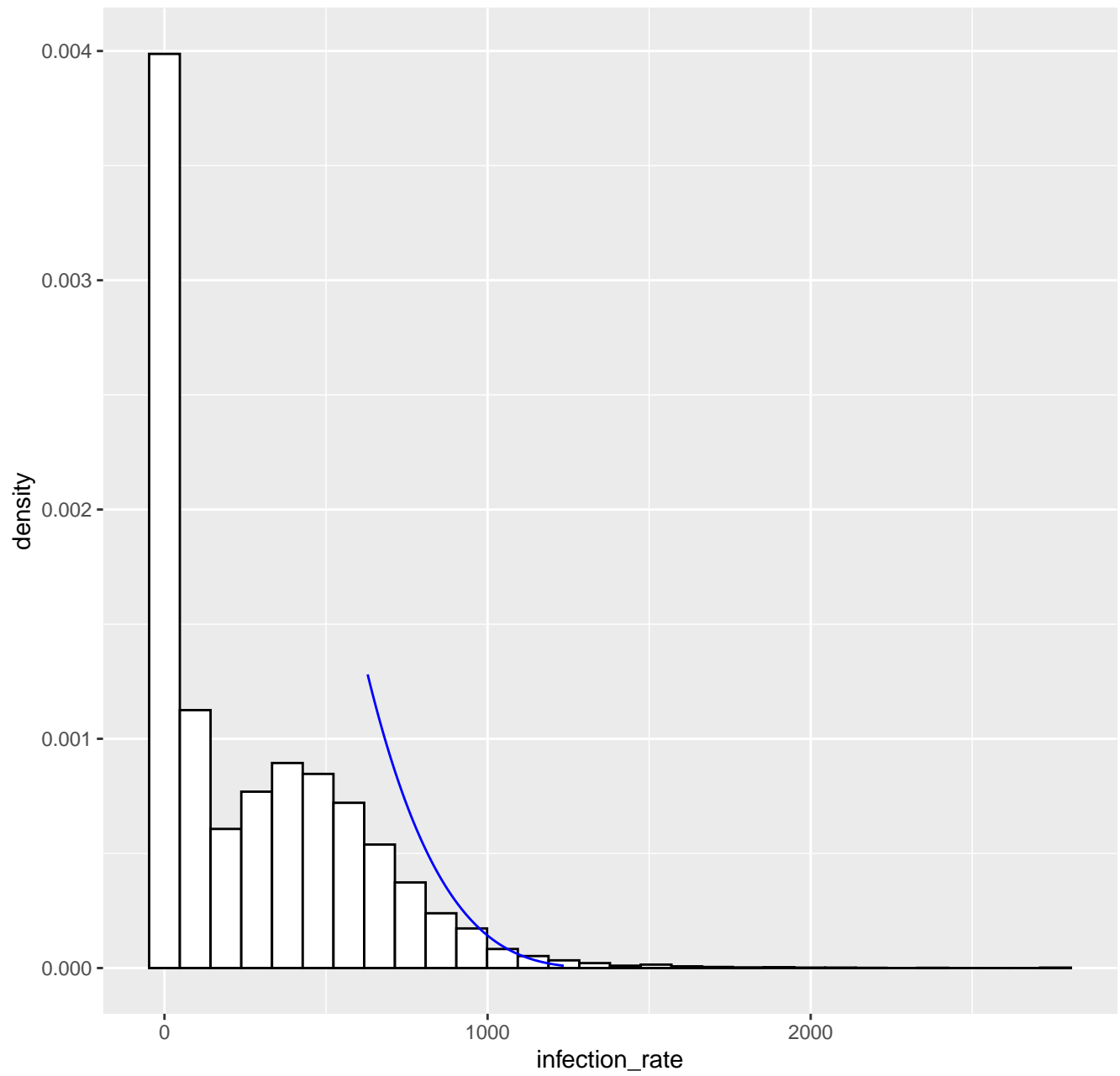
Fitted tail density GPD( 628.8 , 175.95 , -0.21 ), k= 80 -- 11-05-2021
