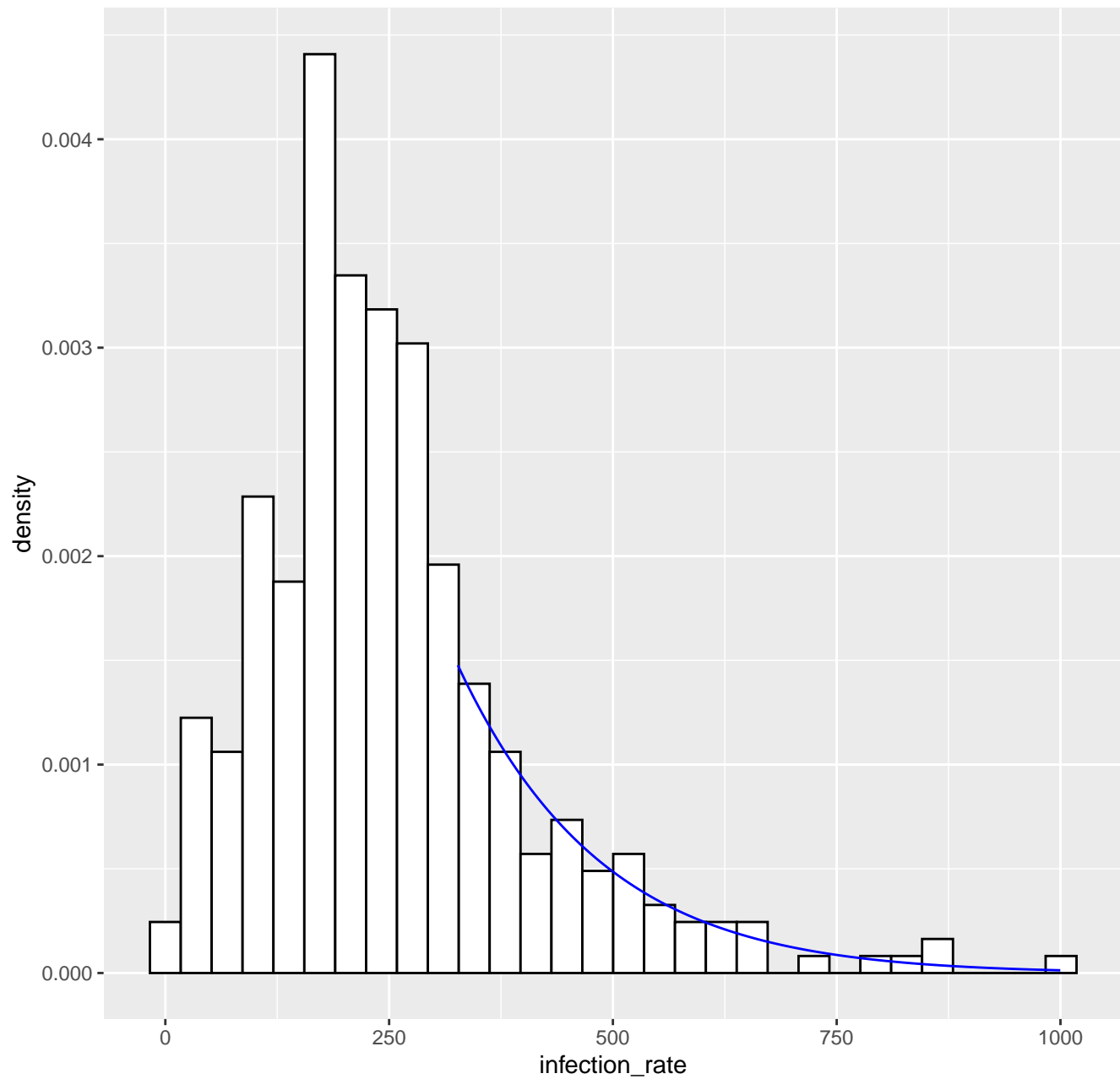
Fitted tail density GPD( 326.8 , 152.61 , -0.05 ), k= 80 -- 11-05-2020
