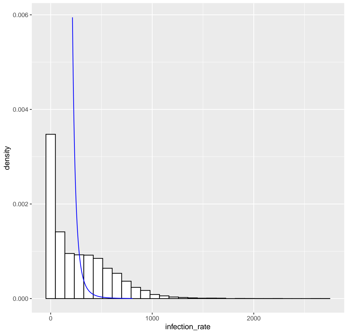
Fitted tail density GPD( 214.7 , 37.89 , 0.28 ), k= 80 -- 10-08-2021
