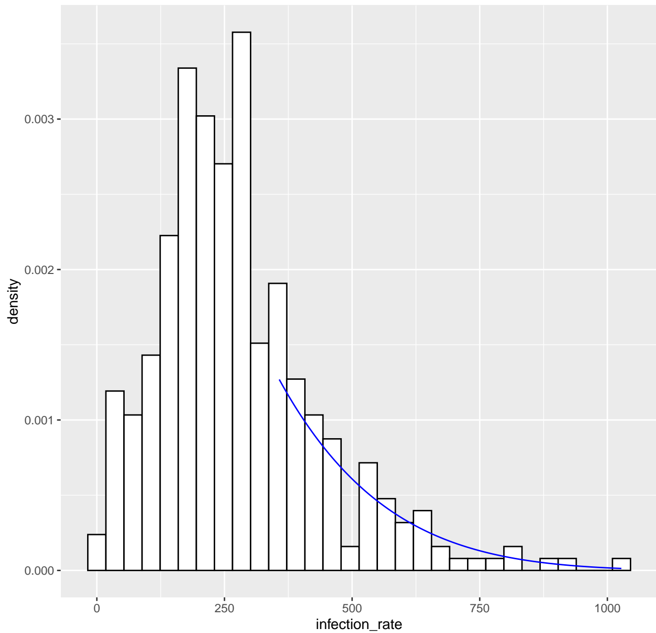
Fitted tail density GPD( 357.3 , 177.57 , -0.14 ), k= 80 -- 10-06-2020
