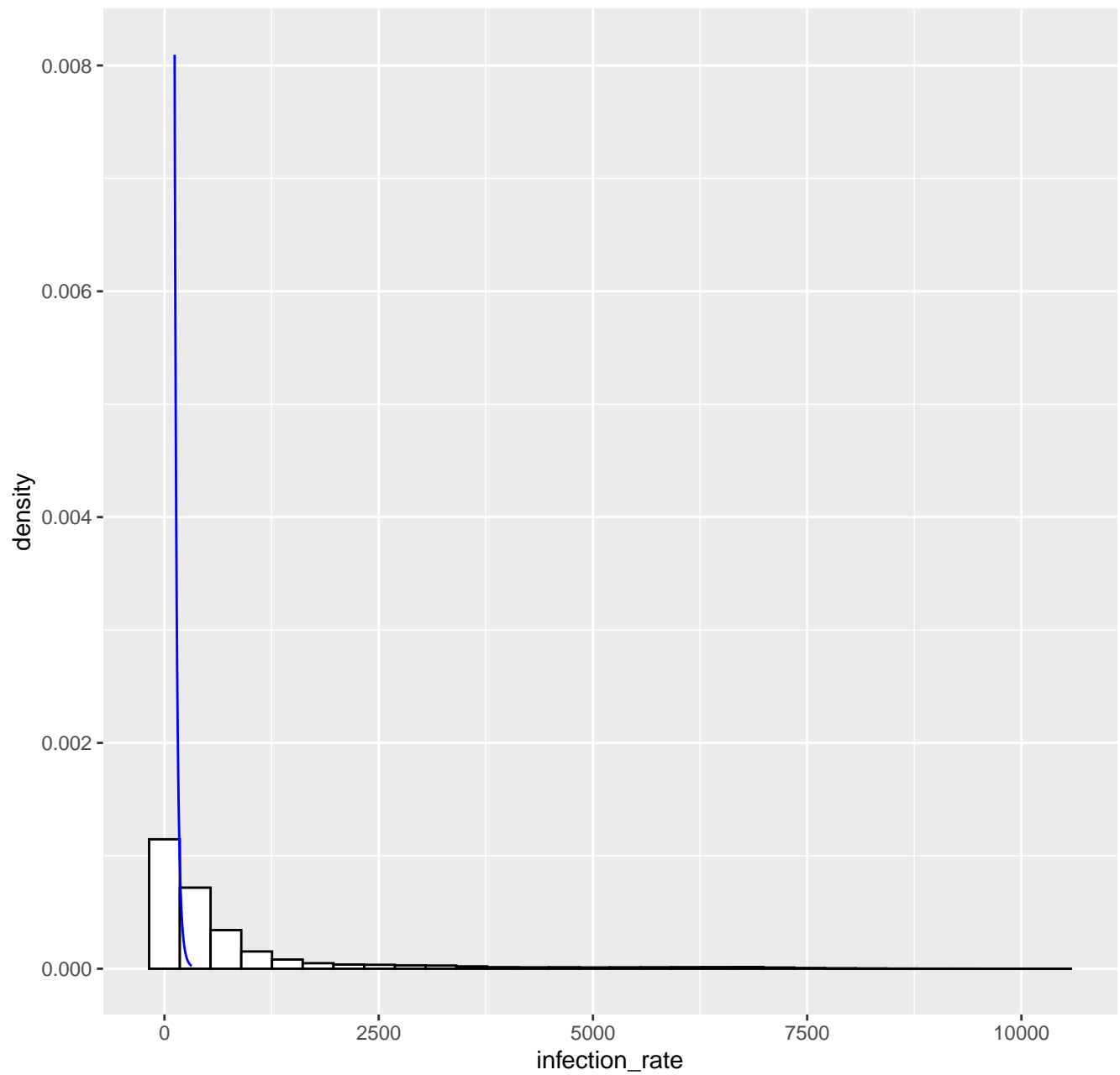
Fitted tail density GPD( 118.5 , 27.84 , 0.12 ), k= 80 -- 10-05-2022
