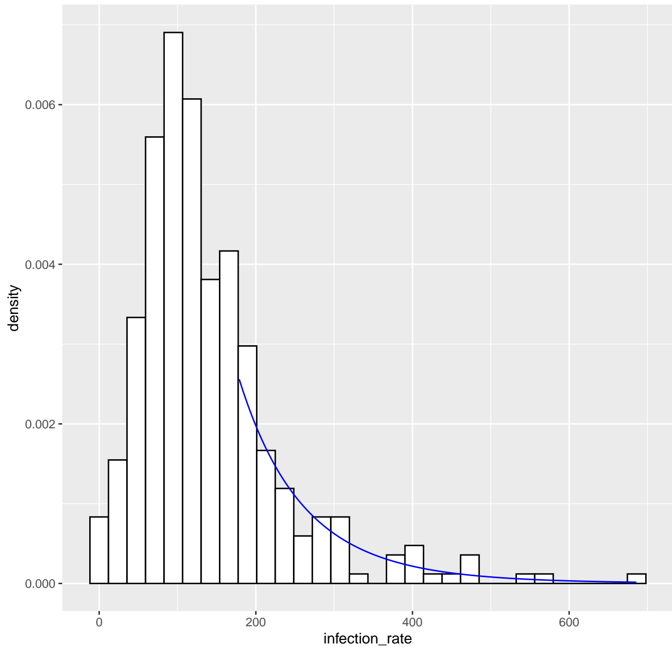
Fitted tail density GPD( 178.8 , 88.06 , 0.08 ), k= 80 -- 10-04-2020
