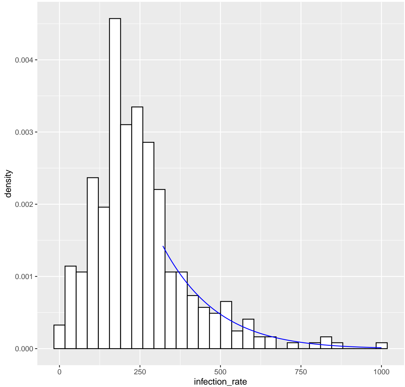
Fitted tail density GPD( 321 , 158.41 , -0.07 ), k= 80 -- 09-05-2020
