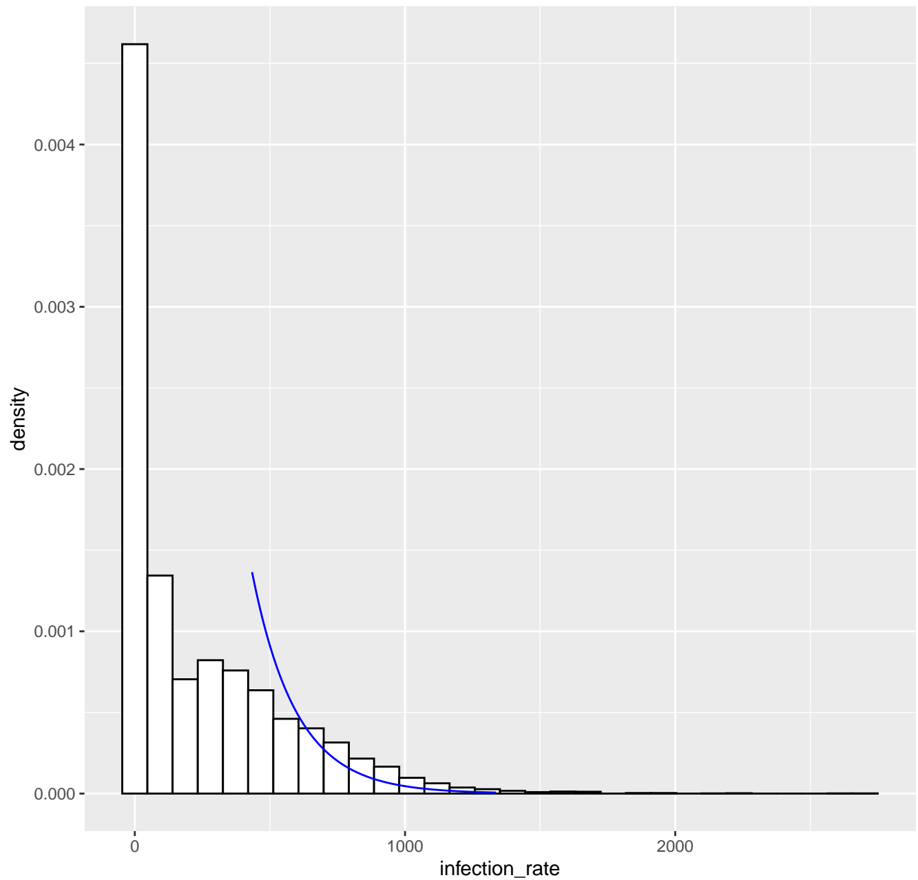
Fitted tail density GPD( 434 , 165.13 , 0.01 ), k= 80 --- 09-03-2021
