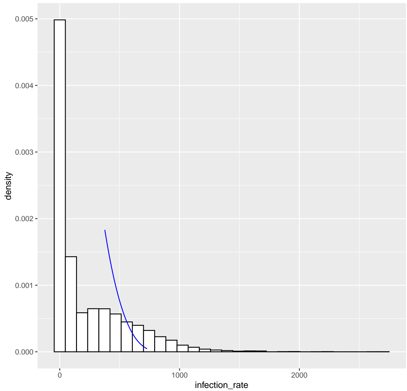
Fitted tail density GPD( 376.1 , 123.09 , -0.24 ), k= 80 -- 09-02-2021
