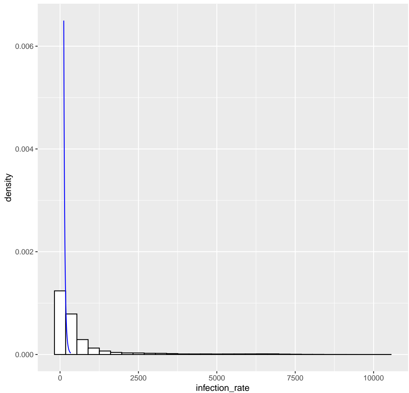
Fitted tail density GPD( 117.9 , 34.68 , 0.09 ), k= 80 -- 08-11-2022
