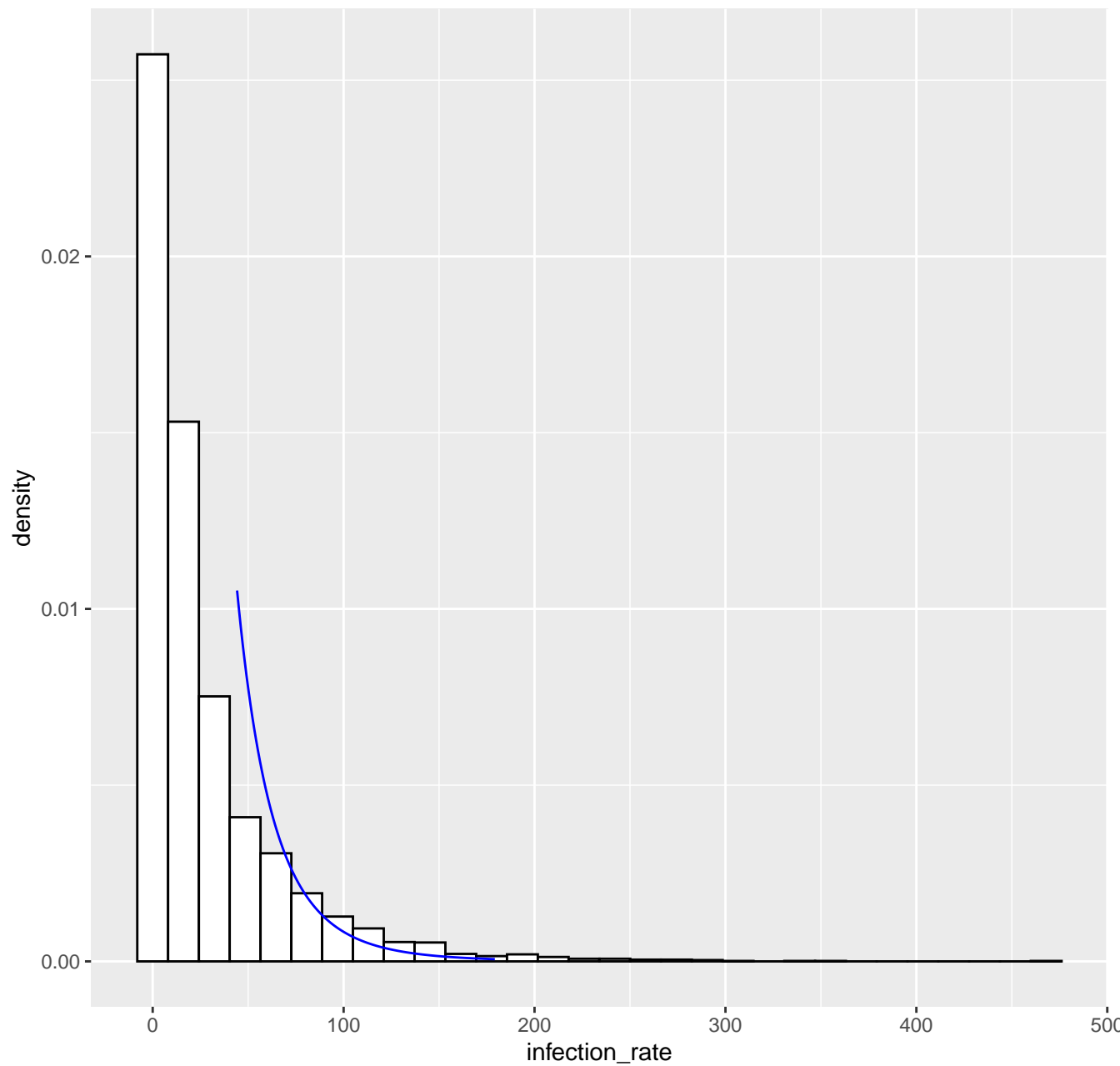
Fitted tail density GPD( 44.2 , 21.42 , 0.15 ), k= 80 -- 08-09-2020
