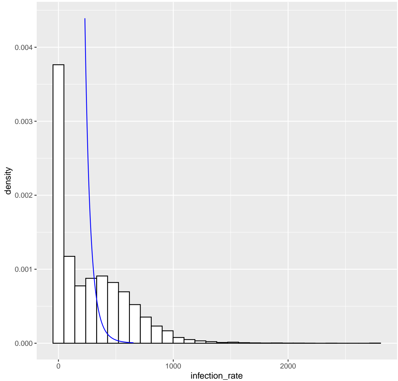
Fitted tail density GPD( 230.3 , 51.32 , 0.11 ), k= 80 -- 08-06-2021
