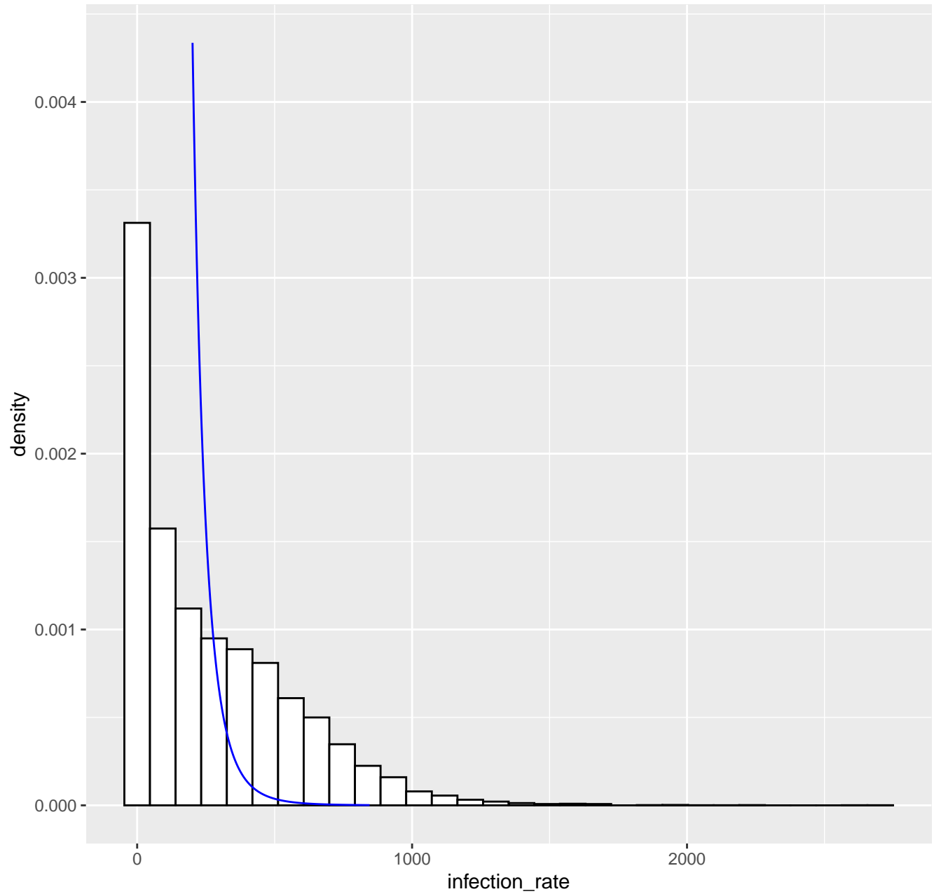
Fitted tail density GPD( 201.4 , 51.97 , 0.15 ), k= 80 -- 07-09-2021
