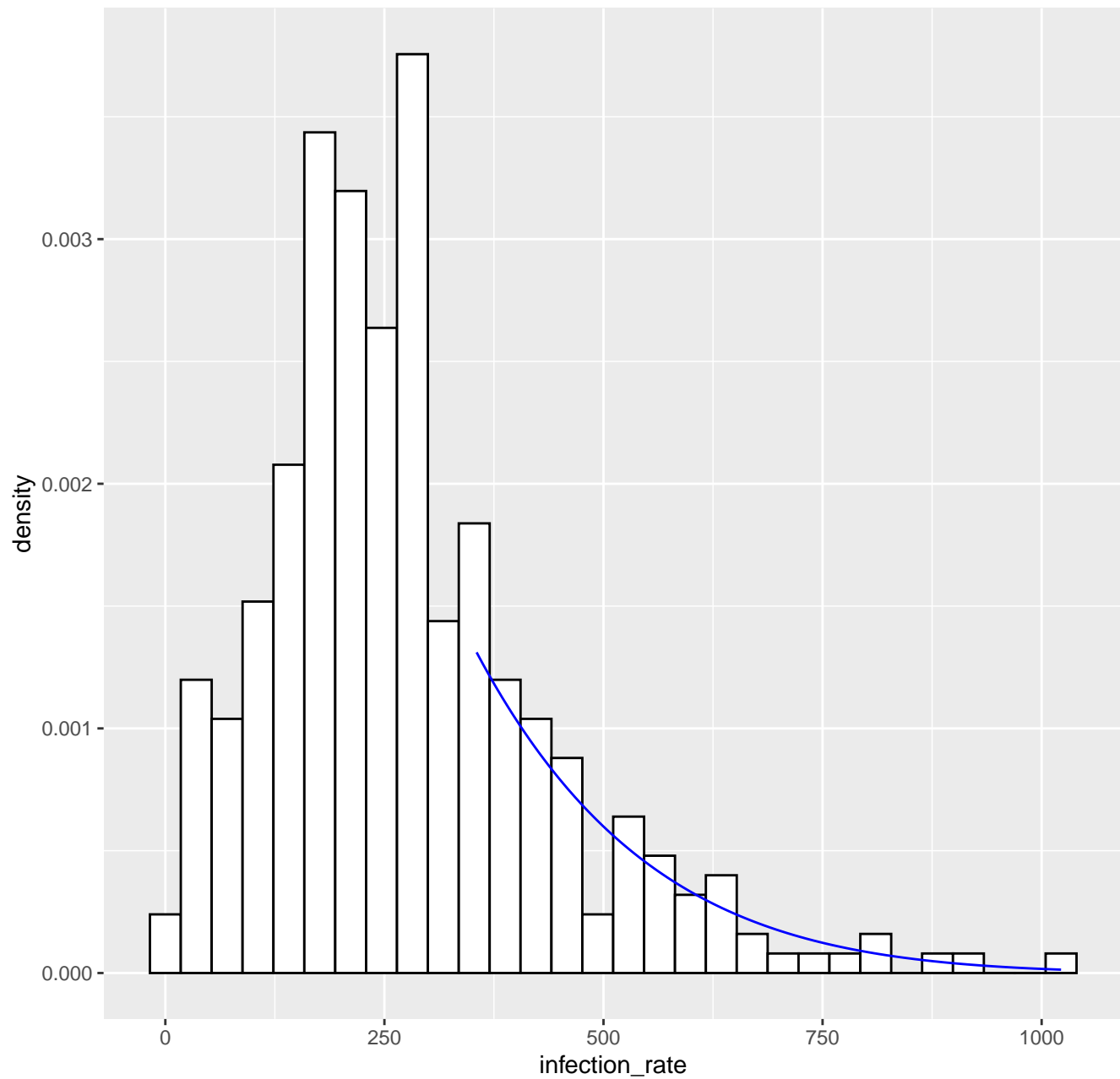
Fitted tail density GPD( 355.2 , 171.9 , -0.12 ), k= 80 -- 07-06-2020
