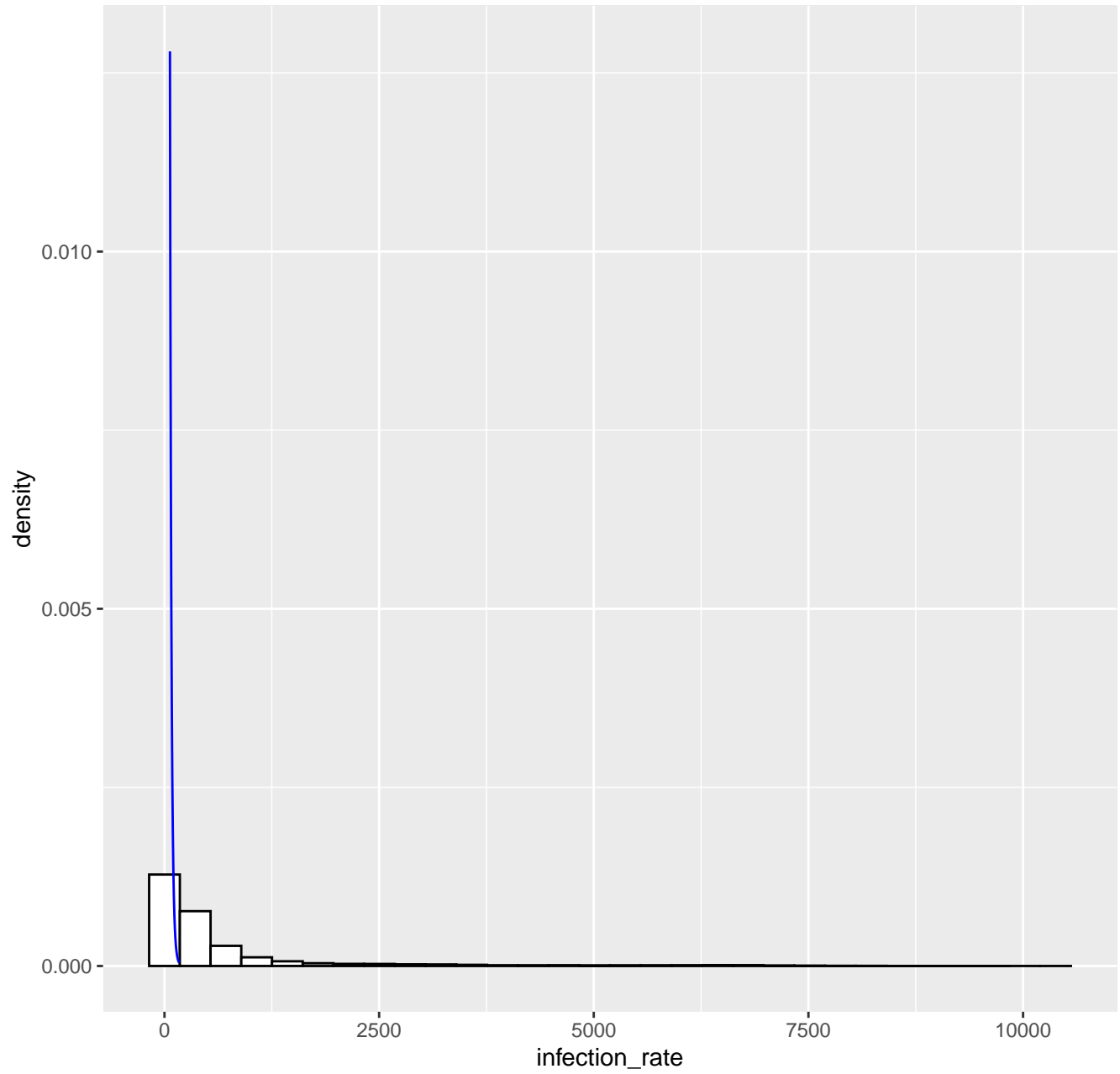
Fitted tail density GPD( 63.6 , 17.6 , 0.04 ), k= 80 -- 06-12-2022
