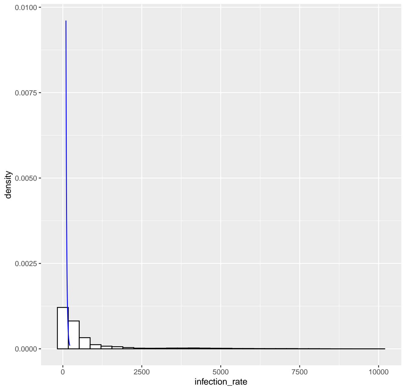
Fitted tail density GPD( 98.5 , 23.45 , 0.1 ), k= 80 -- 06-09-2022
