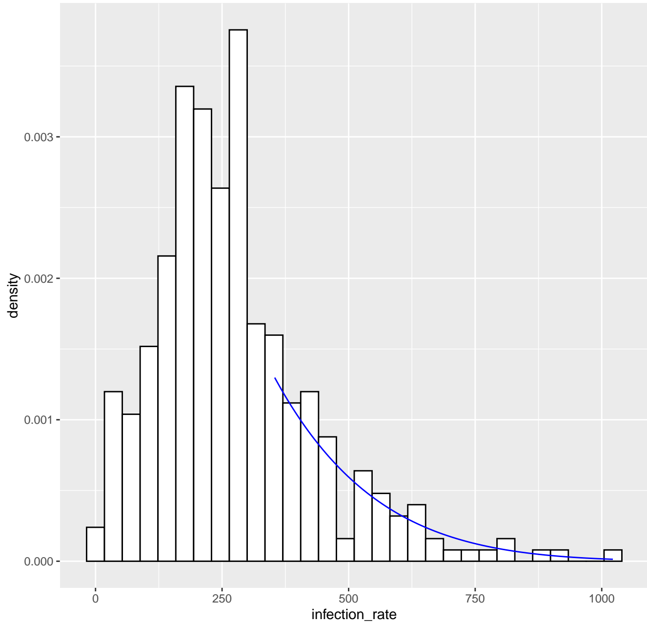
Fitted tail density GPD( 354 , 173.61 , -0.12 ), k= 80 -- 06-06-2020
