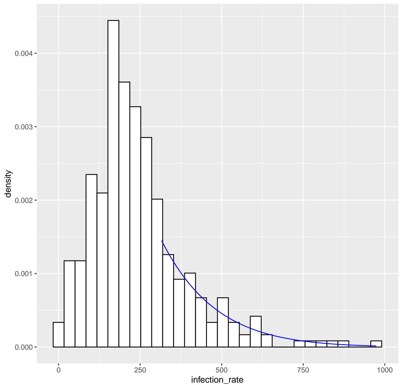
Fitted tail density GPD( 315.8 , 155.54 , -0.06 ), k= 80 -- 06-05-2020
