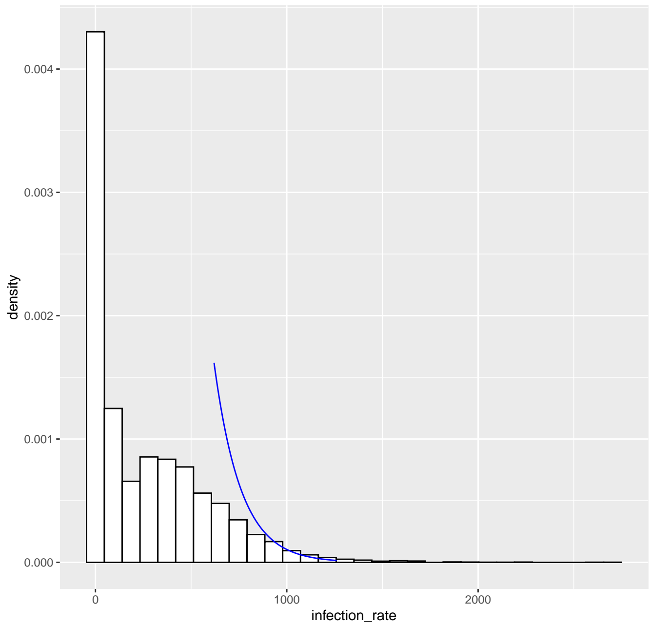
Fitted tail density GPD( 619.8 , 139.23 , -0.01 ), k= 80 -- 06-04-2021
