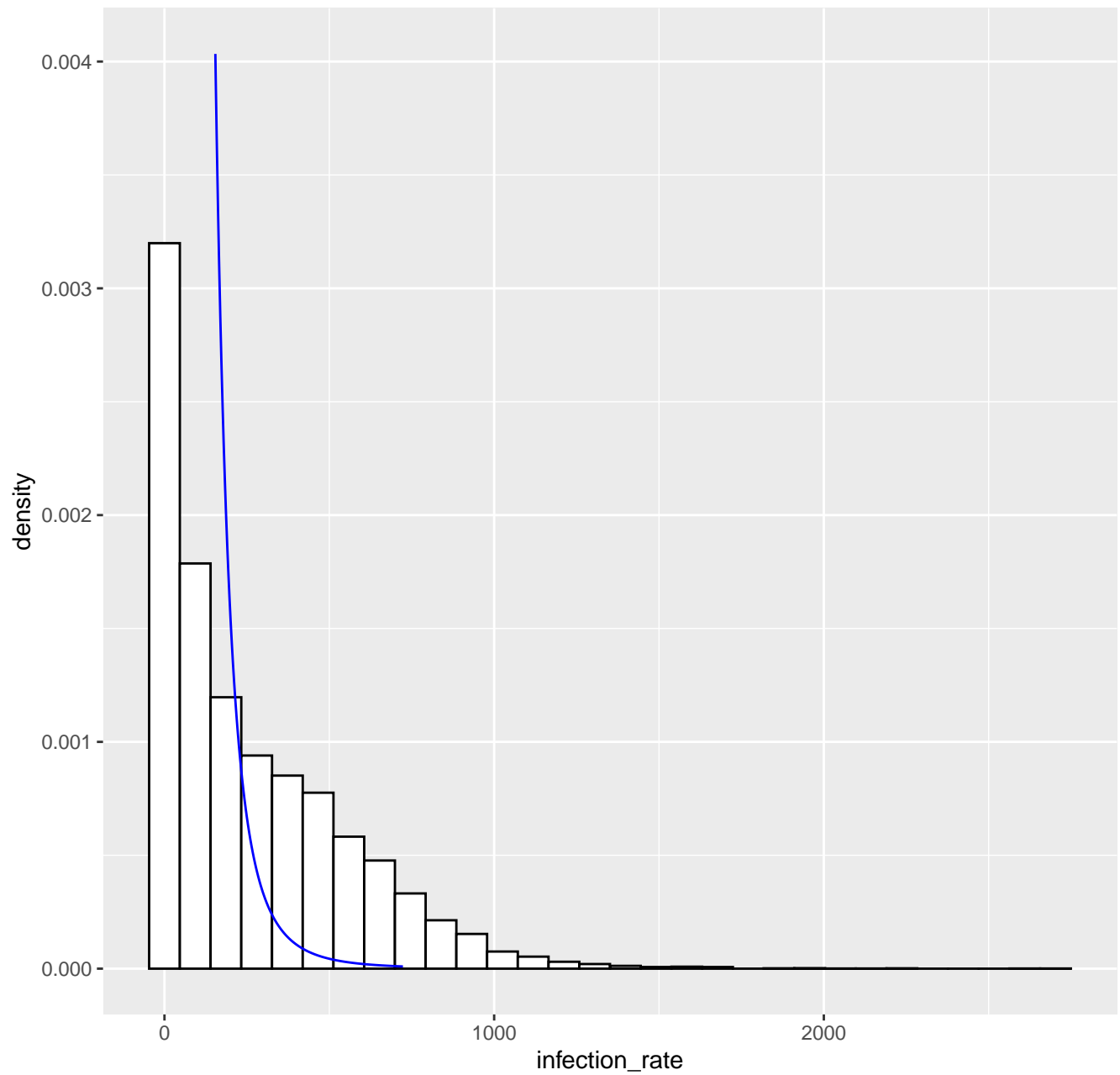
Fitted tail density GPD( 154.3 , 55.87 , 0.31 ), k= 80 -- 05-10-2021
