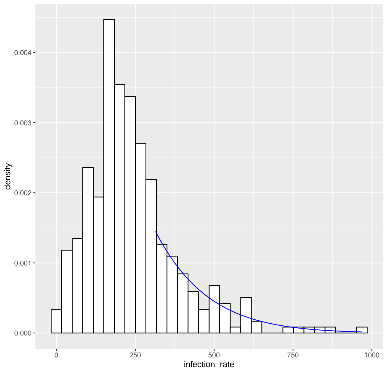
Fitted tail density GPD( 314.3 , 155.52 , -0.06 ), k= 80 -- 05-05-2020
