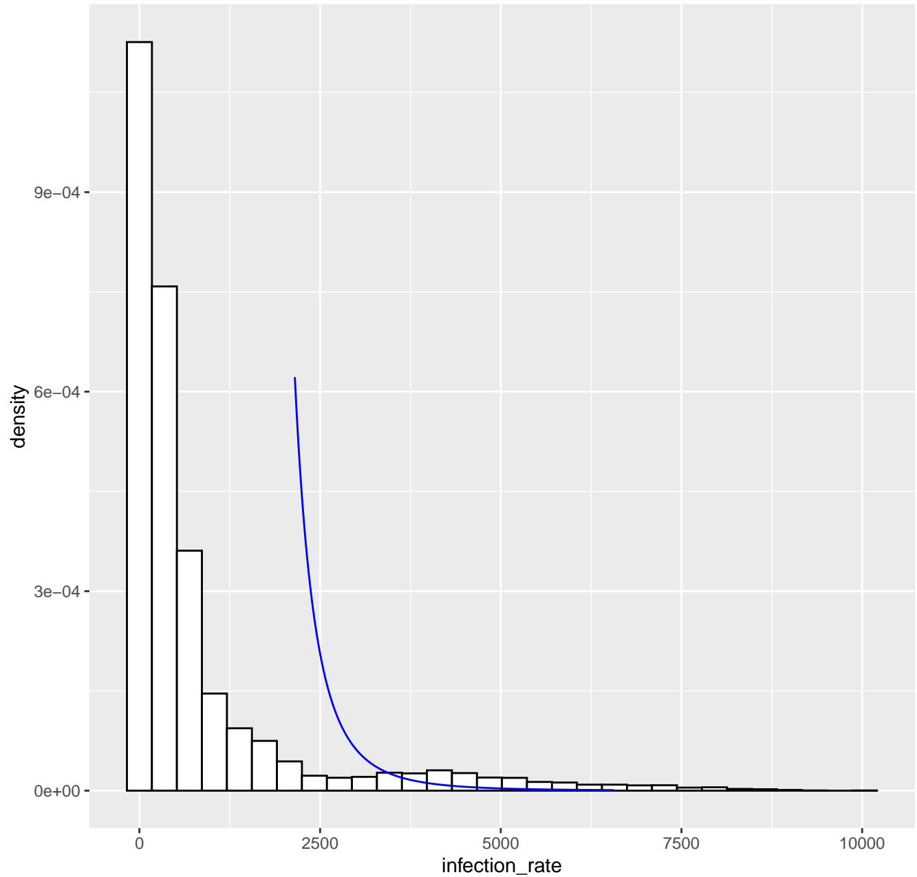
Fitted tail density GPD( 2150.4 , 362.39 , 0.31 ), k= 80 -- 05-04-2022
