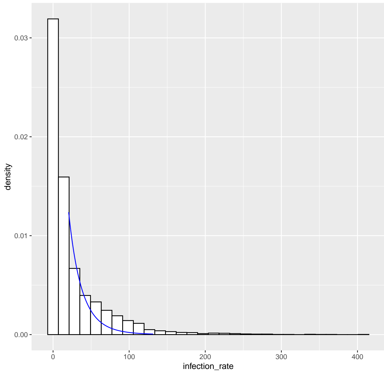
Fitted tail density GPD( 20.5 , 18.22 , 0.08 ), k= 80 -- 04-08-2020
