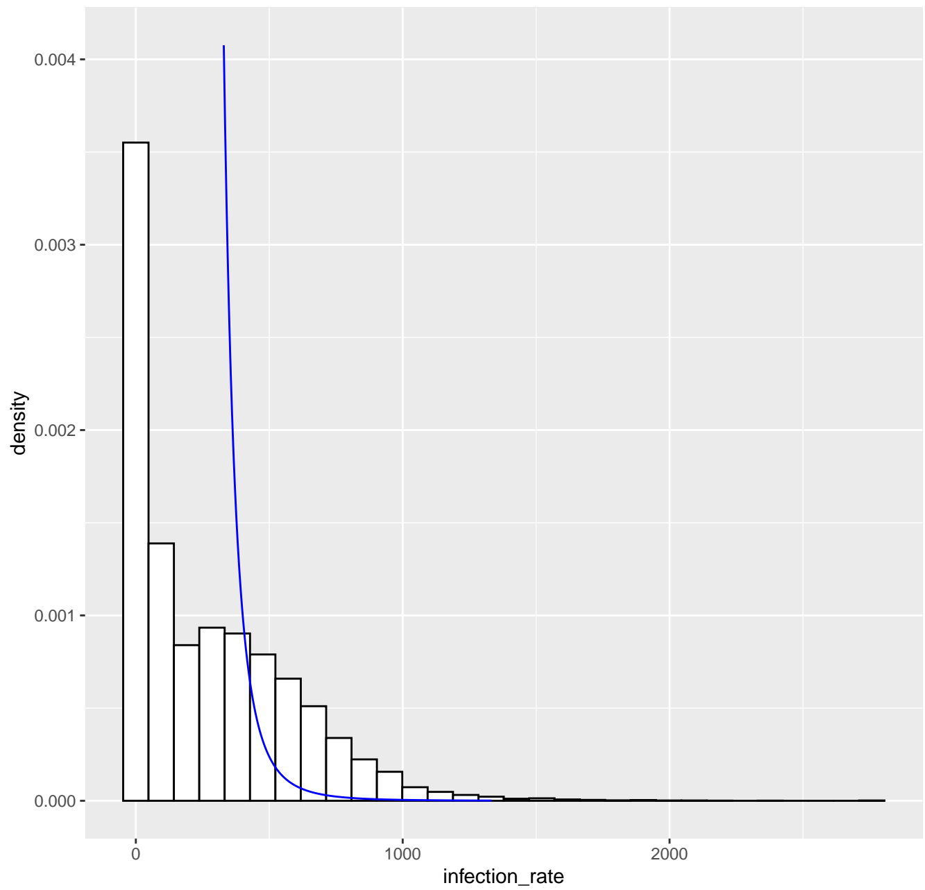
Fitted tail density GPD( 329.6 , 55.28 , 0.29 ), k= 80 -- 03-08-2021
