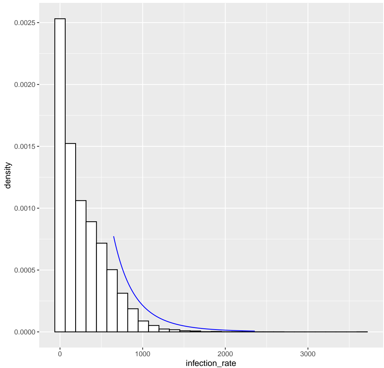
Fitted tail density GPD( 648.7 , 291.45 , 0.17 ), k= 80 -- 02-11-2021
