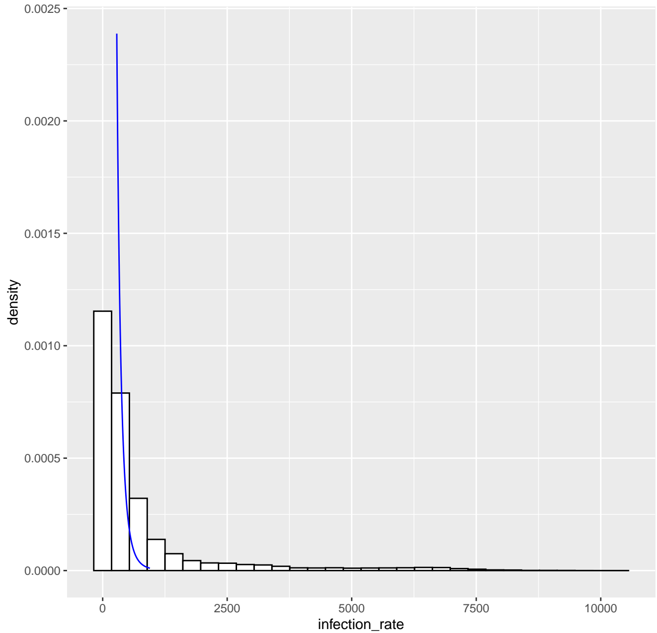
Fitted tail density GPD( 283.5 , 94.36 , 0.17 ), k= 80 -- 02-08-2022
