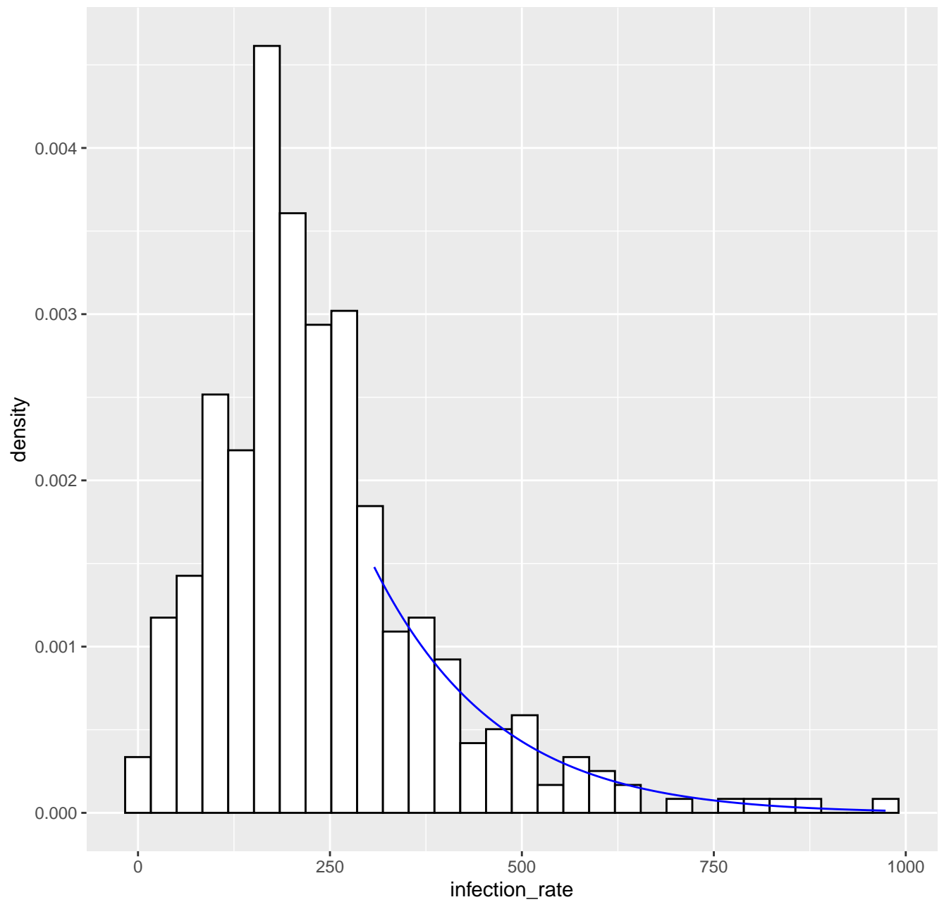
Fitted tail density GPD( 307.7 , 152.4 , -0.05 ), k= 80 --- 02-05-2020
