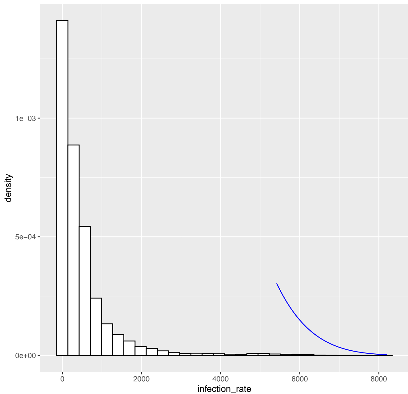
Fitted tail density GPD( 5416.4 , 741.8 , -0.15 ), k= 80 -- 02-02-2022
