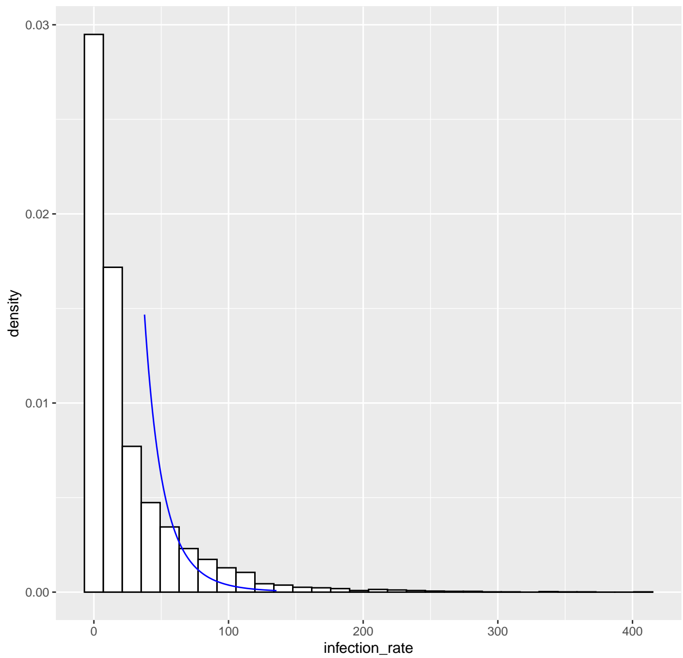
Fitted tail density GPD( 37.6 , 15.36 , 0.14 ), k= 80 -- 01-09-2020
