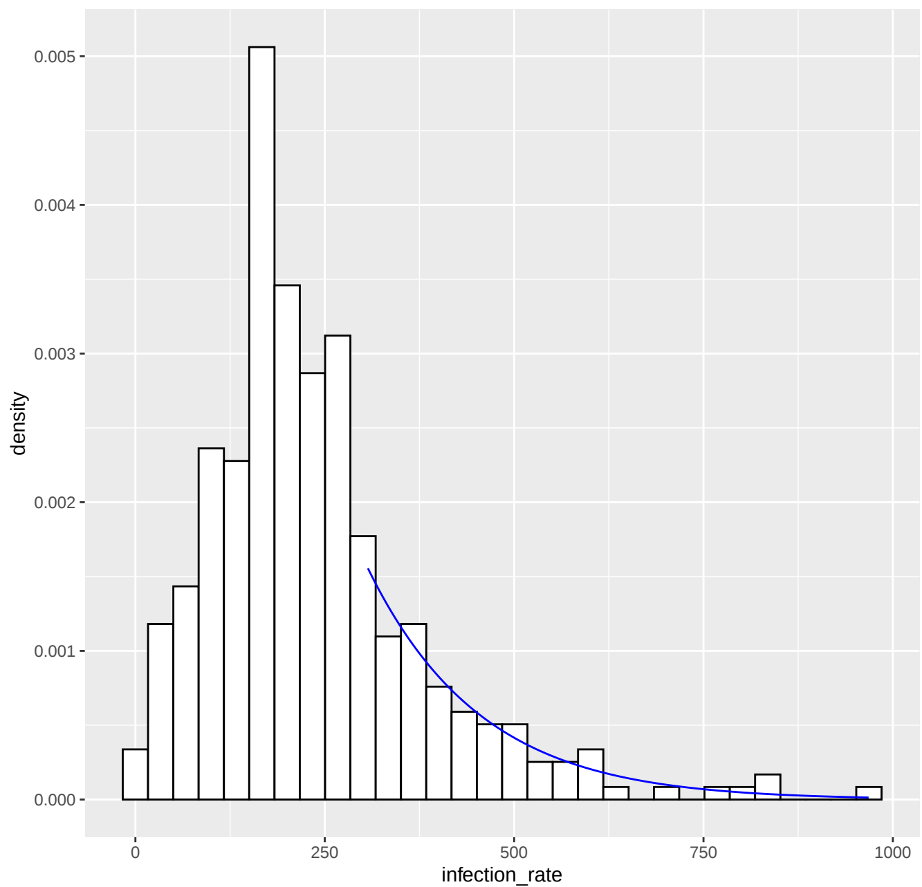
Fitted tail density GPD( 307 , 144.88 , -0.03 ), k= 80 -- 01-05-2020
