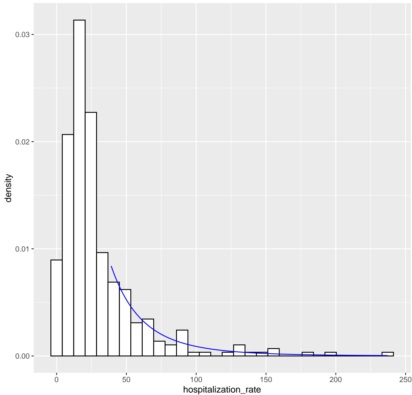
Fitted tail density GPD( 39.1 , 26.83 , 0.2 ), k= 80 --- 31-03-2020
