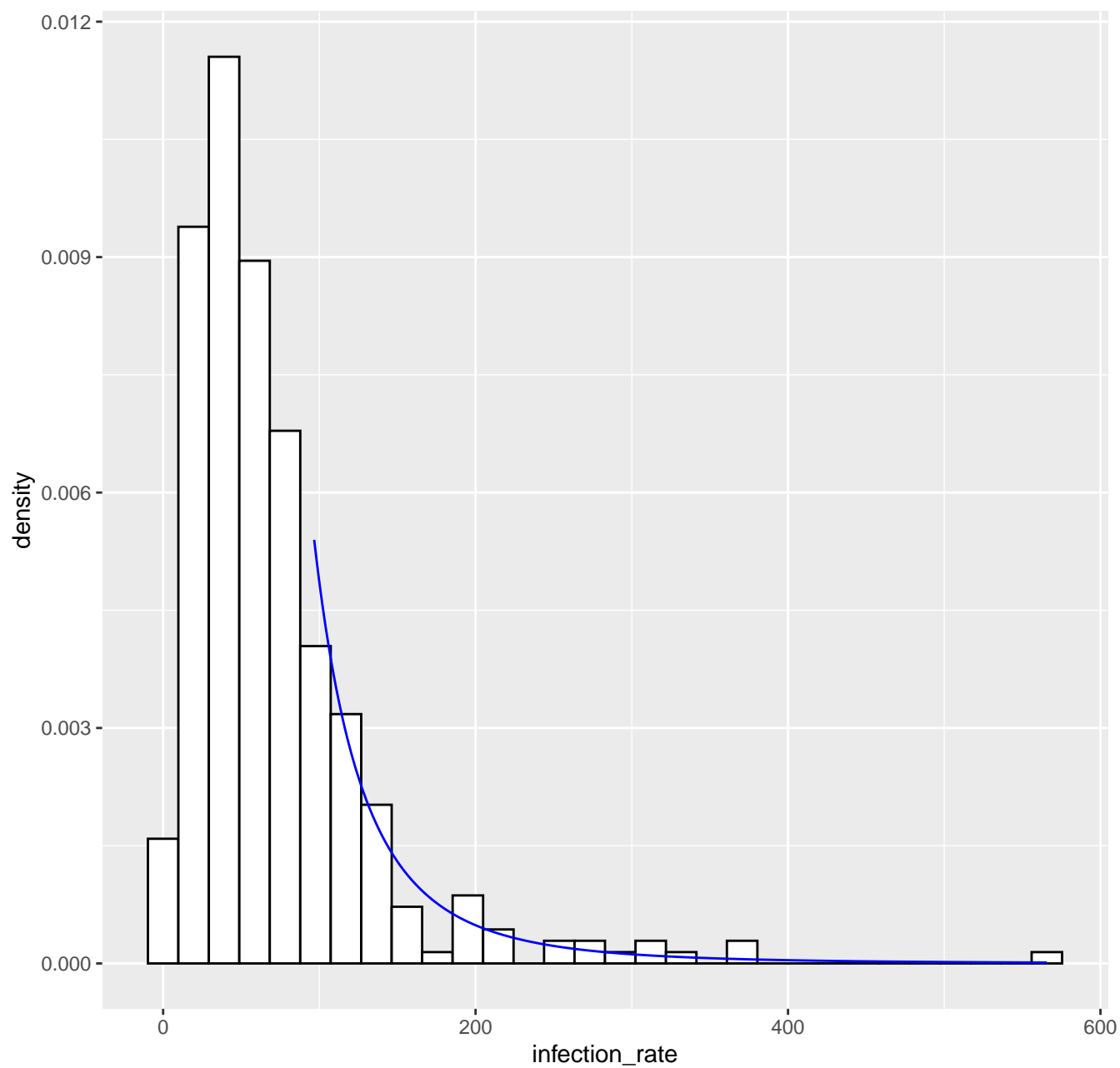
Fitted tail density GPD( 96.7 , 41.75 , 0.35 ), k= 80 -- 30-03-2020
