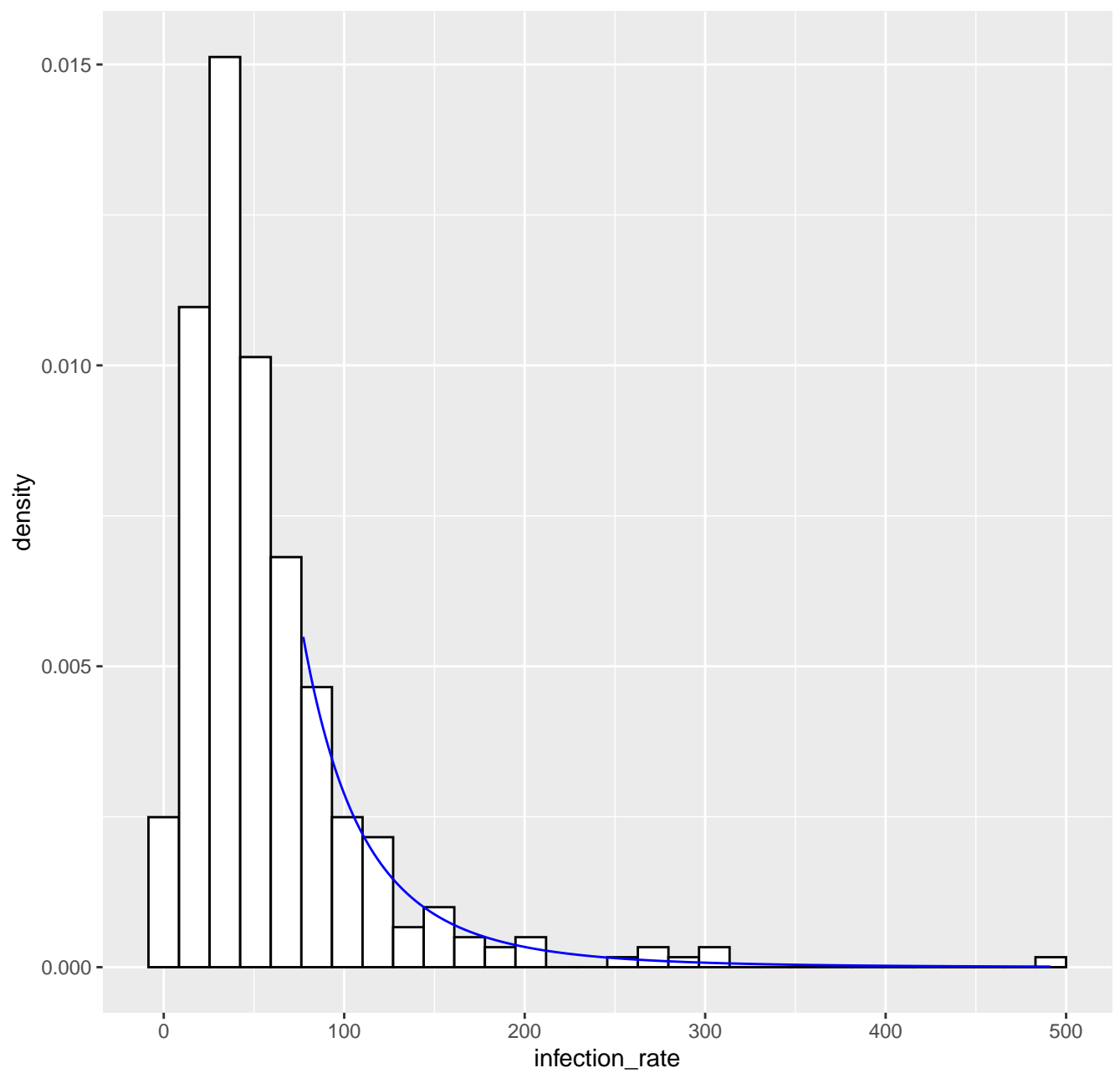
Fitted tail density GPD( 77.3 , 41.05 , 0.25 ), k= 80 -- 28-03-2020
