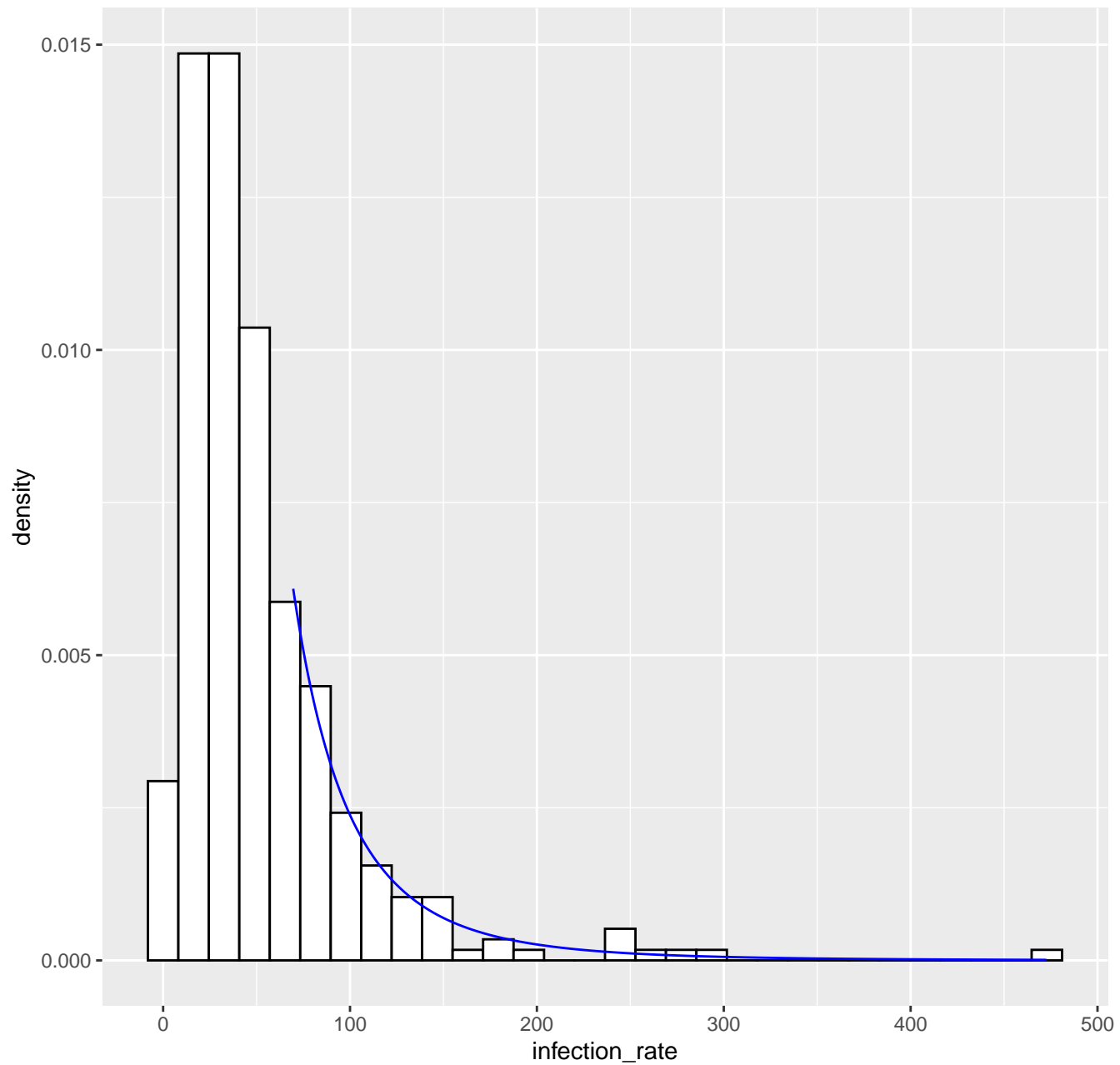
Fitted tail density GPD( 69.6 , 37.02 , 0.26 ), k= 80 -- 27-03-2020
