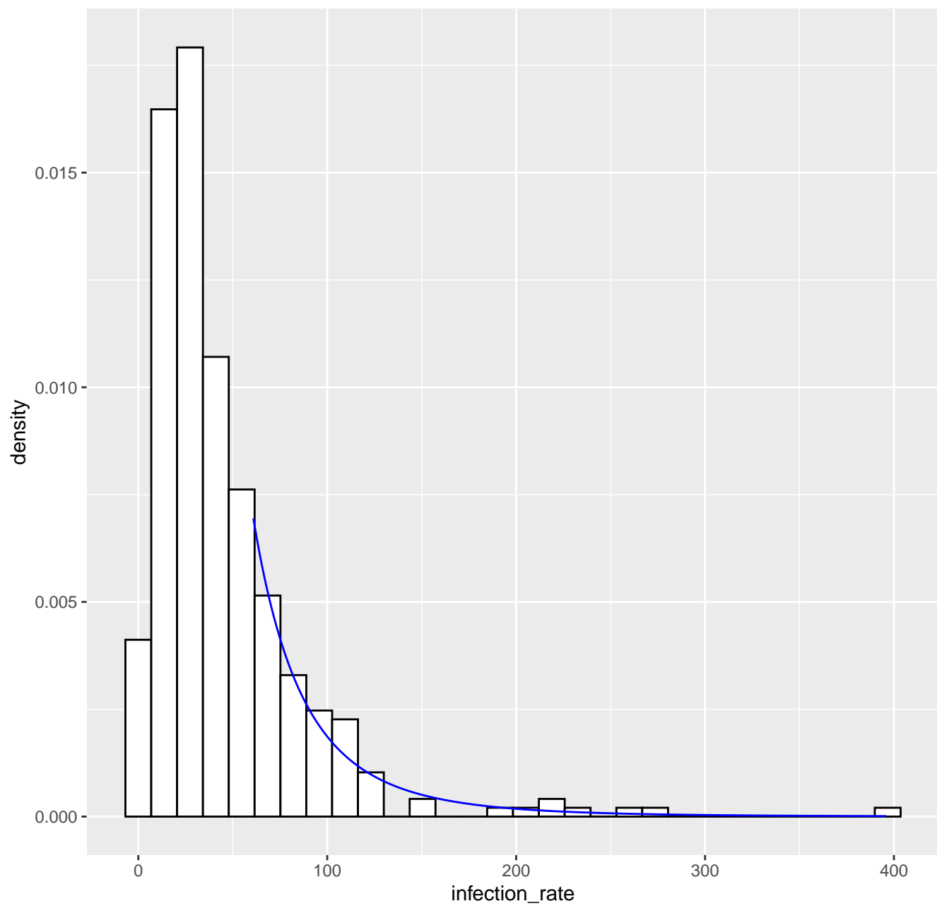
Fitted tail density GPD( 60.9 , 32.45 , 0.25 ), k= 80 -- 26-03-2020
