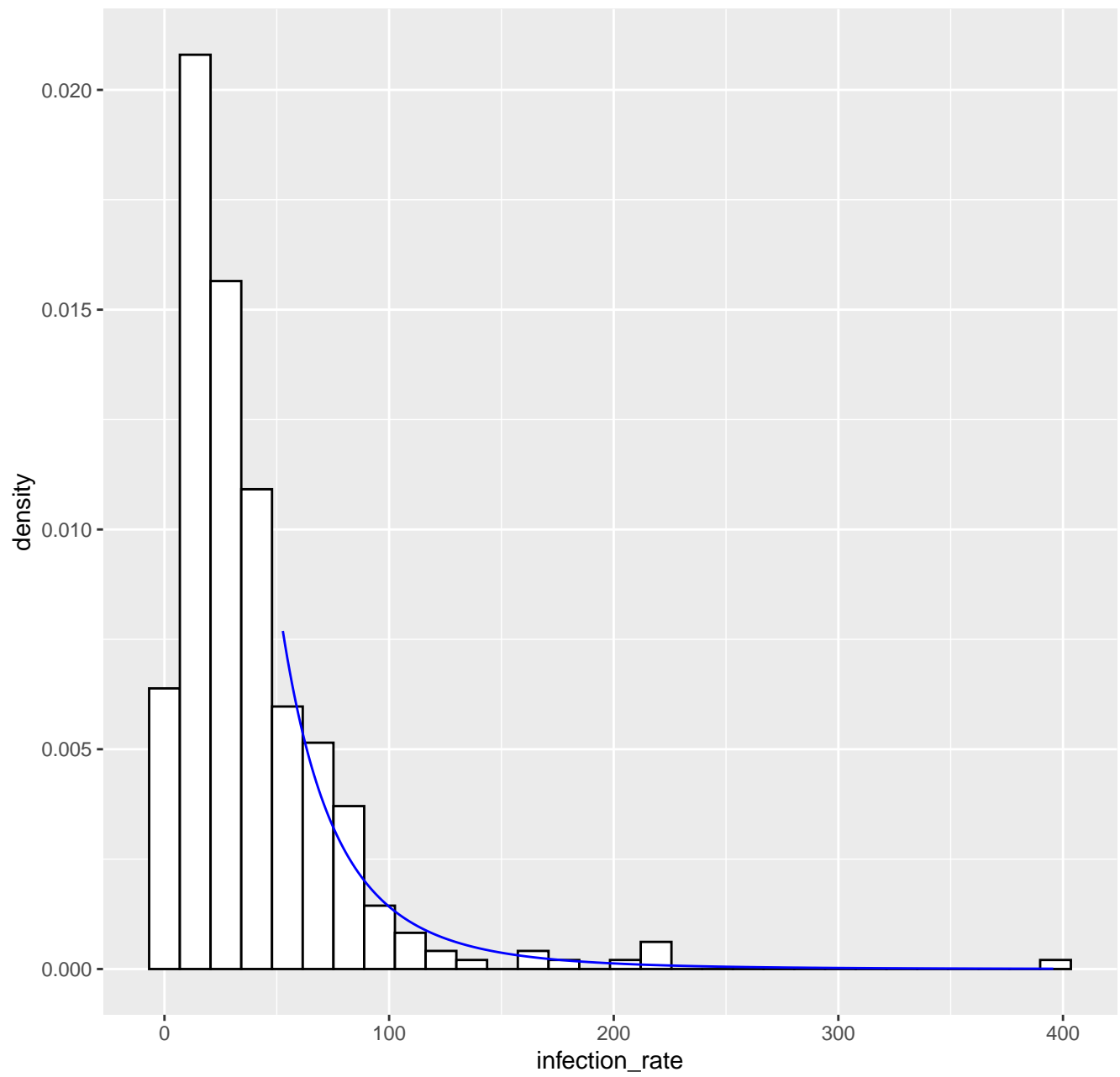
Fitted tail density GPD( 52.69 , 29.3 , 0.23 ), k= 80 -- 25-03-2020
