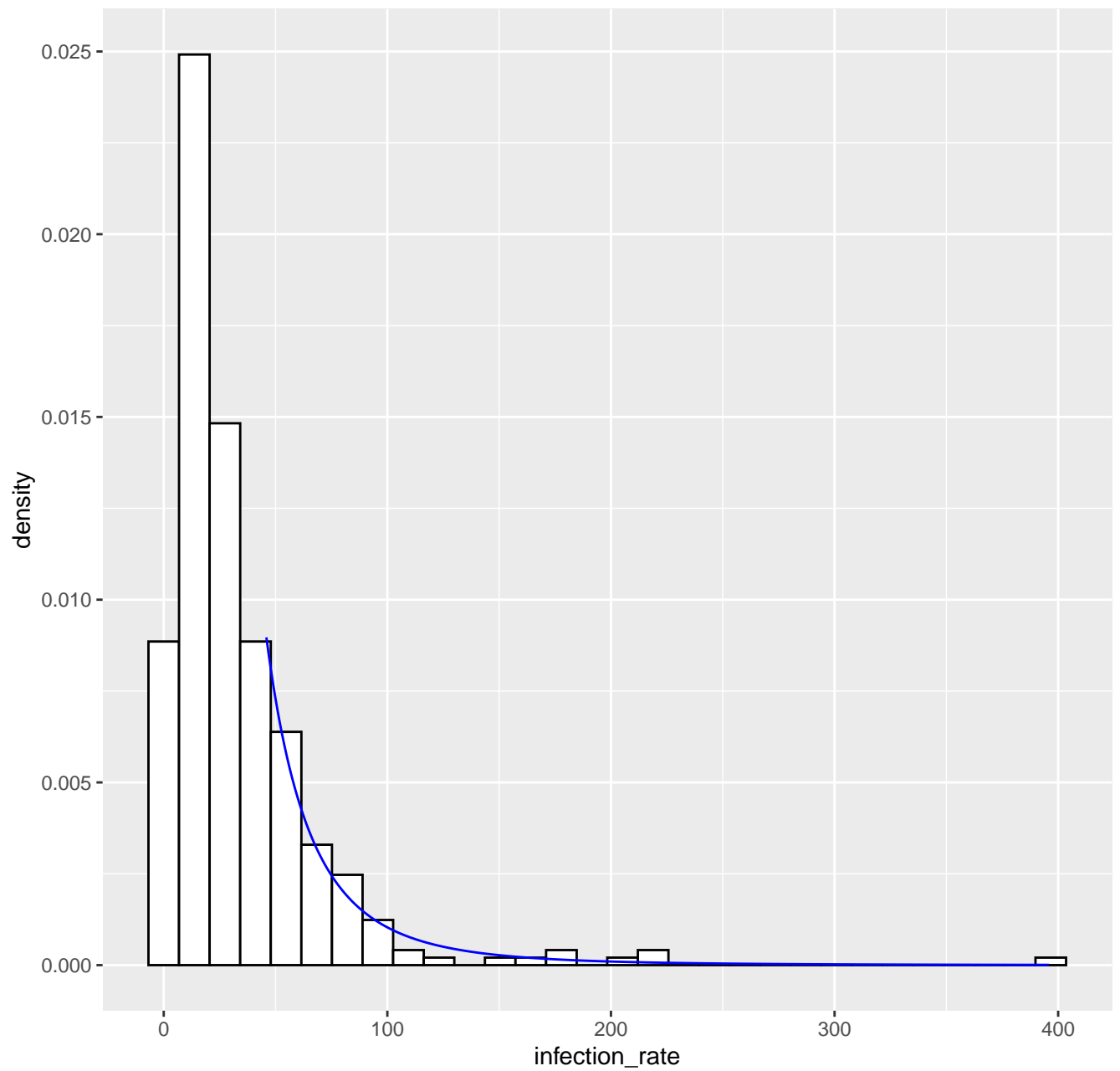
Fitted tail density GPD( 45.9 , 25.13 , 0.31 ), k= 80 -- 24-03-2020
