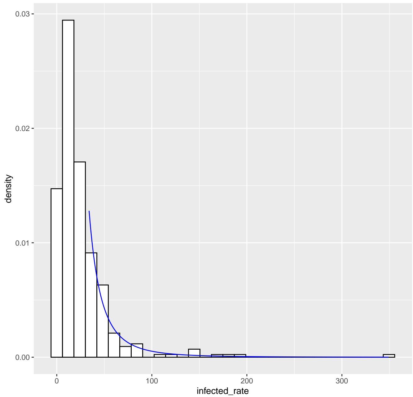
Fitted tail density GPD( 34 , 17.61 , 0.42 ), k= 80 -- 22-03-2020
